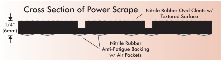
Anti-Fatigue backing
